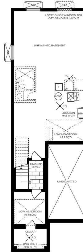
ELEVATION A & B Basement For Opt. Sec Floor with 4 Bedrooms
