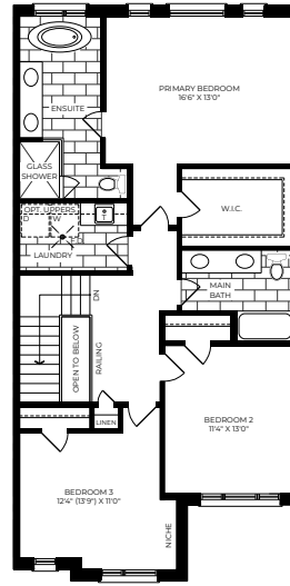
ELEVATION A Second Floor
