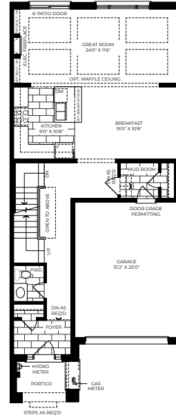
ELEVATION A Ground Floor
