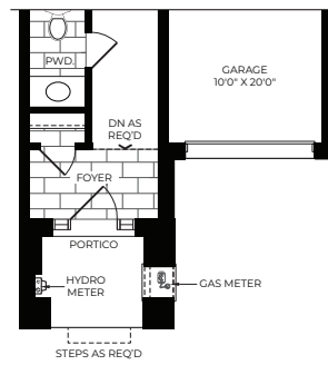
ELEVATION B Ground Floor
