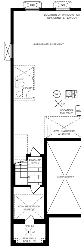
ELEVATION A & B Basement
