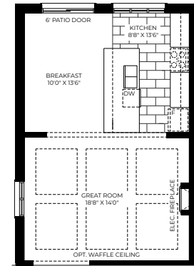
LAYOUT 1 Opt. Ground Floor
