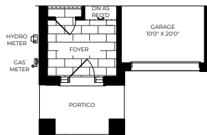
ELEVATION B Ground Floor
