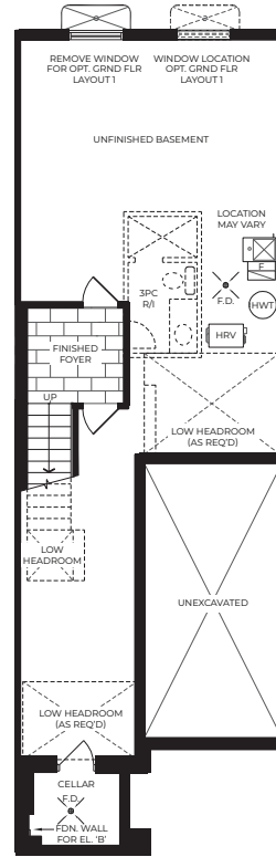
ELEVATION A & B Basement
