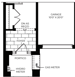
ELEVATION B Ground Floor
