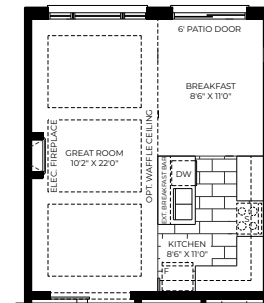
LAYOUT 2 Opt. Ground Floor
